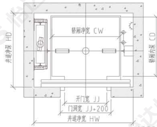
井道平面布置图 (中分门) Shaft plan view (center opening)
