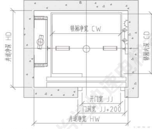
井道平面布置图 (旁开门) Shaft plan view (two panel side opening)
