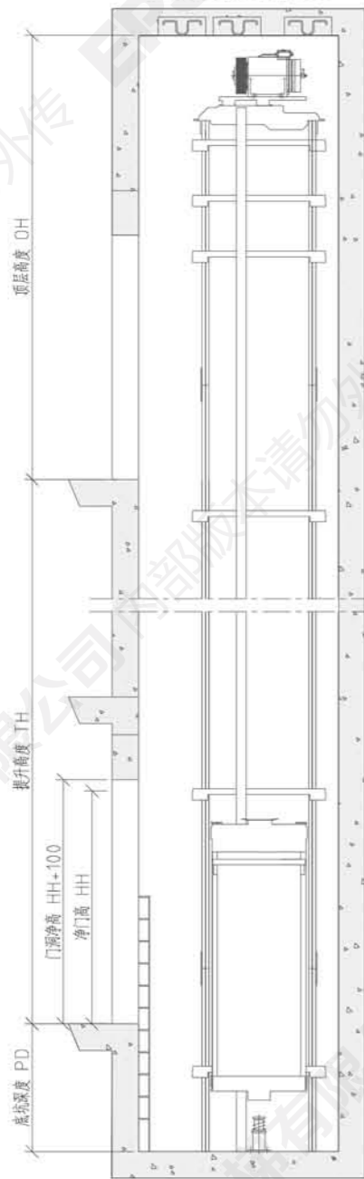
井道立面布置图 Shaft elevation plan view
