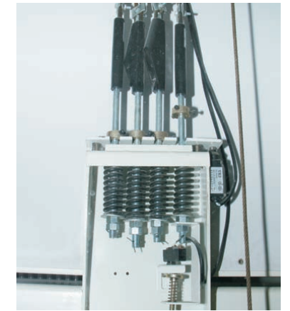
断绳开关 Rope Broken Switch
