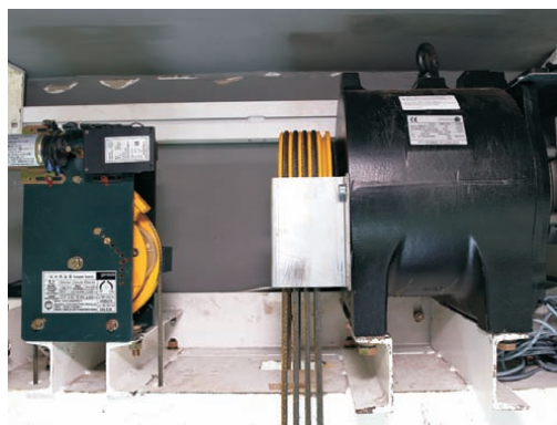
曳引机 Traction machine
